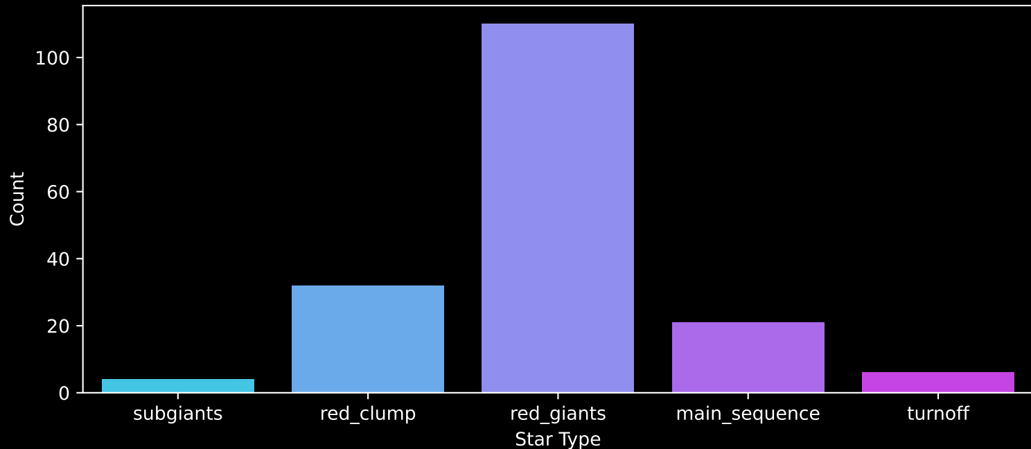
APOGEE DR17 Field: [240+12] Count plot of Star Type
