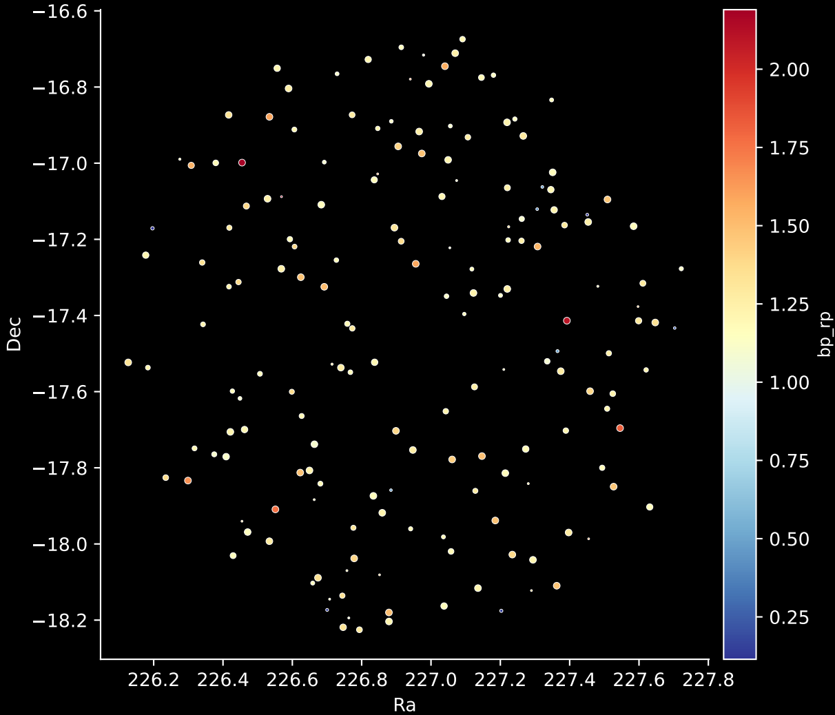
APOGEE DR17 Field: [240+12] Stars: 173
