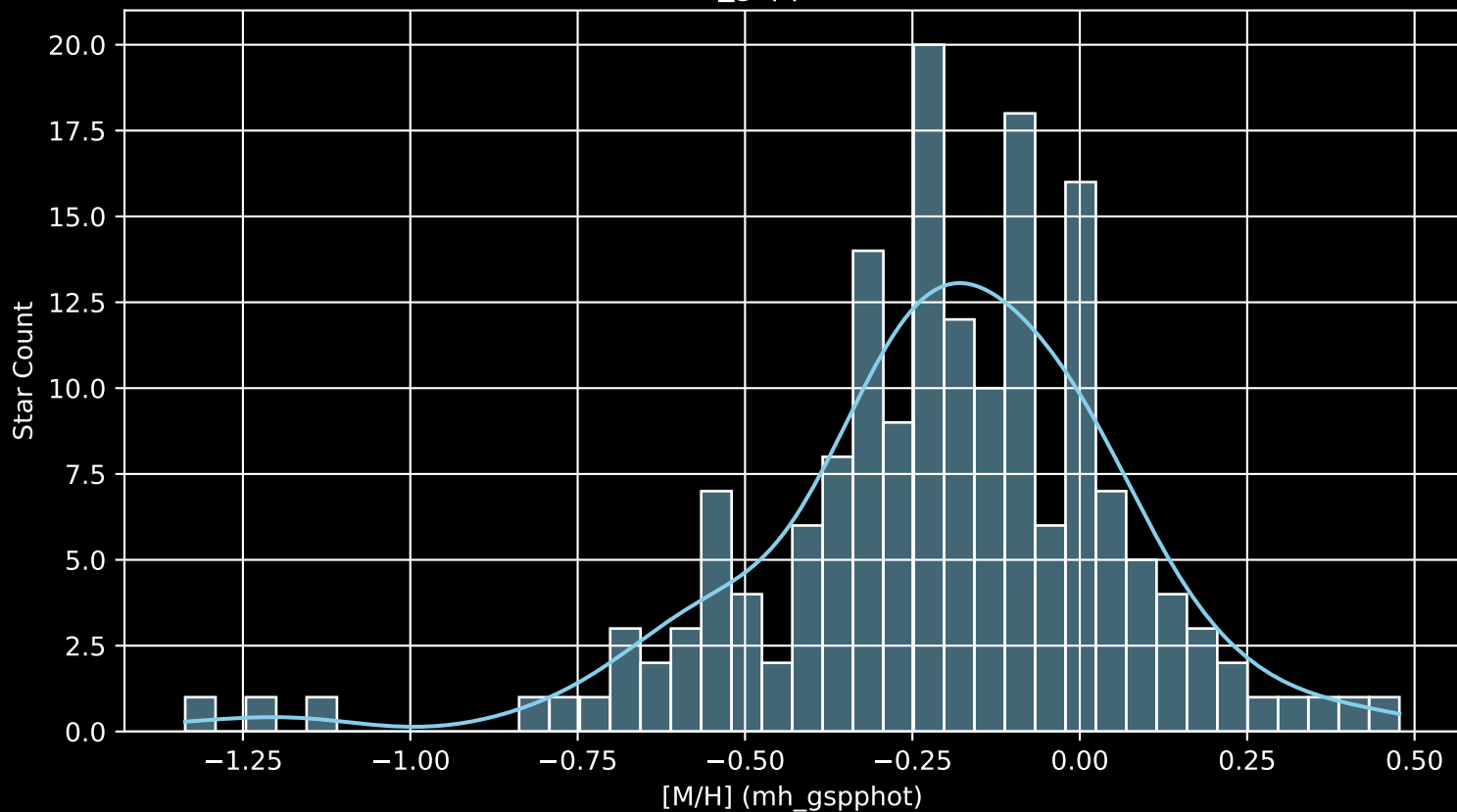
APOGEE DR17 Field: [240+12 [M/H] (mh_gspphot) (n= 172)
