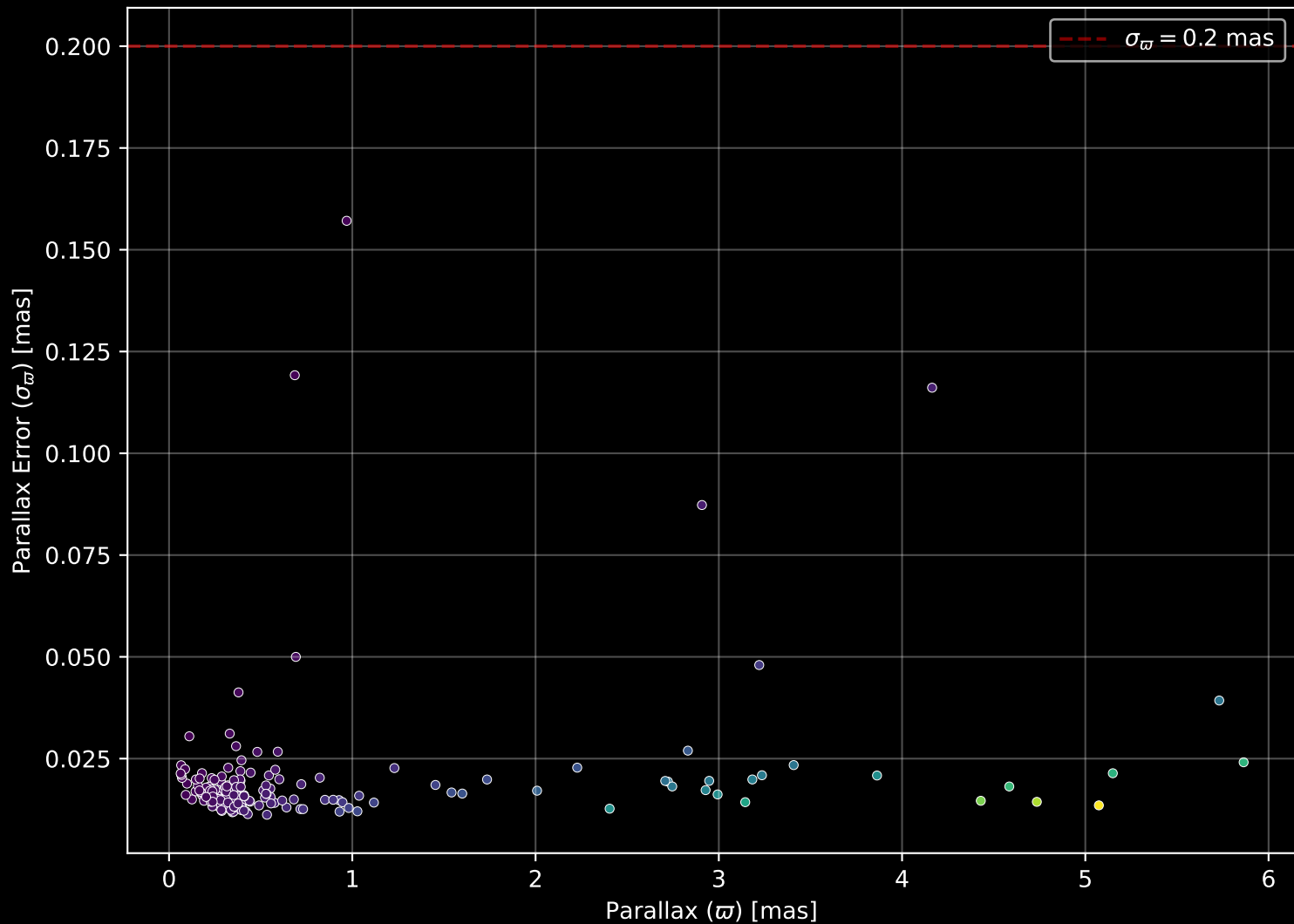
APOGEE DR17 Field: [240+12] Parallax Quality (n= 173)
