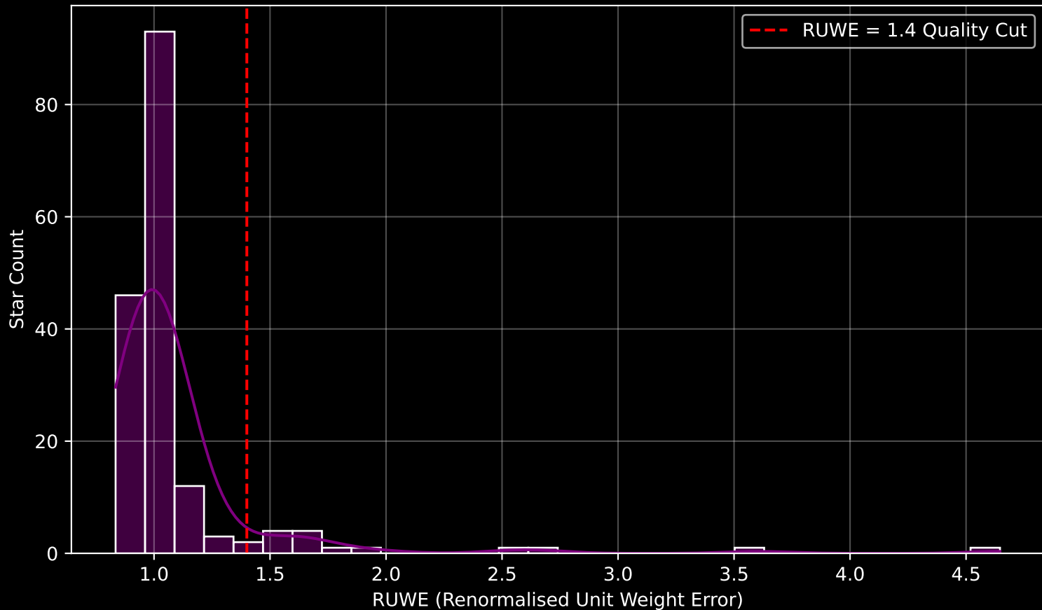
GAPOGEE DR17 Field [240+12] RUWE Distribution (n= 170)
