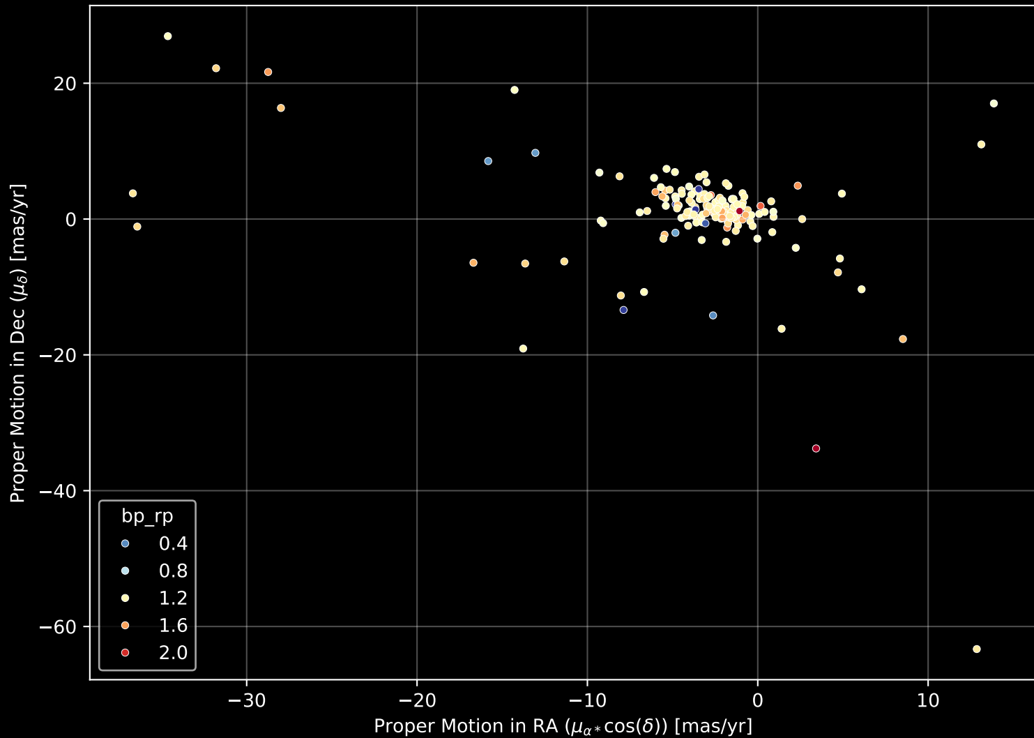
APOGEE DR17 Field: [240+12] Proper Motion Diagram (n= 173)
